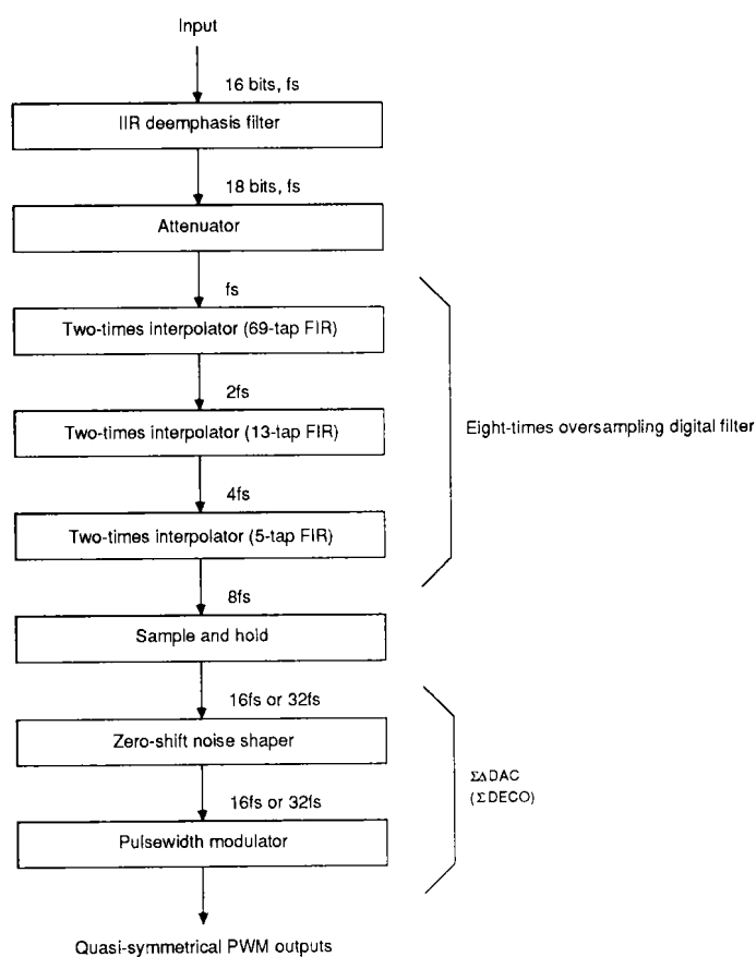
Figure 1. Arithmetic operation
