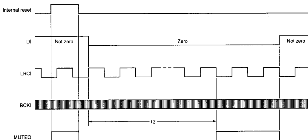
Figure 15. MUTEO output waveforms
