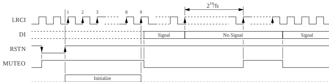
Figure 2. MUTEO output timing
