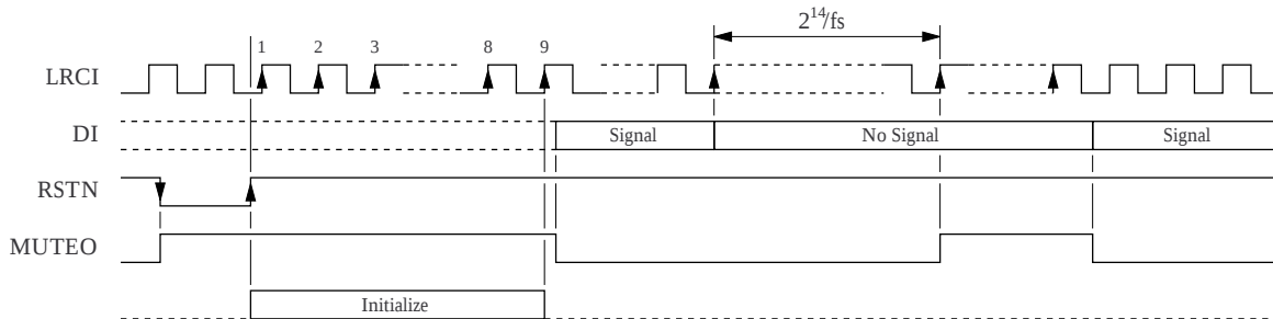
Figure 3. MUTEO output timing
