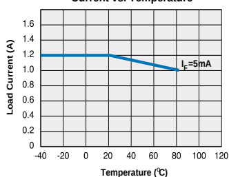
CPC1945Y Typical Maximum Load Current vs. Temperature
