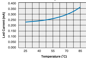
CPC1945Y Typical I_F for Switch Operation Over Temperature
