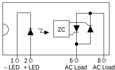
CPC1965Y Pinout
