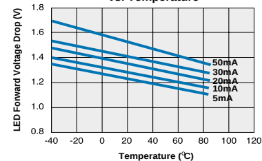
CPC1965Y Typical LED Forward Voltage Drop vs. Temperature
