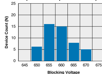
CPC1965Y Typical Blocking Voltage Distribution (Ambient Temperature = 25°C)
