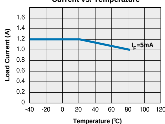
CPC1965Y Typical Maximum Load Current vs. Temperature
