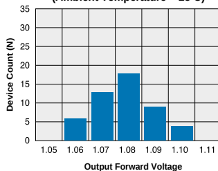
CPC1965Y Typical On-State Output Forward Voltage Distribution (Ambient Temperature = 25°C)
