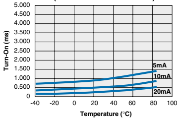
IAA110P Typical Turn-On vs. Temperature (Load Current = 100mADC)
