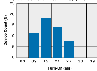
IAA110P Typical Turn-On Time (N=50 Ambient Temperature = 25°C) (Load Current = 100mADC; I_F = 5mADC)
