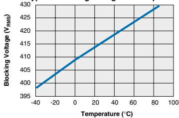
IAA110P Typical Blocking Voltage vs. Temperature
