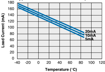
IAA110P Typical Load Current vs. Temperature
