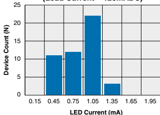
LBA110L - FormA Typical I_F for Switch Dropout (N=50 Ambient Temperature = 25°C) (Load Current = 120mADC)
