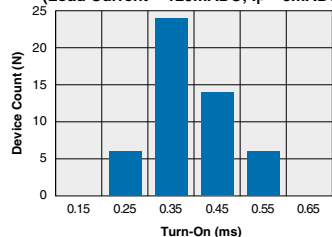
LBA110L - FormA Typical Turn-On Time (N=50 Ambient Temperature = 25°C) (Load Current = 120mADC; I_F = 5mADC)
