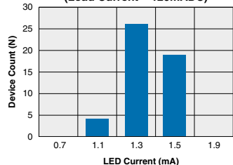
LBA110L - FormB Typical I_F for Switch Operation (N=50 Ambient Temperature = 25°C) (Load Current = 120mADC)
