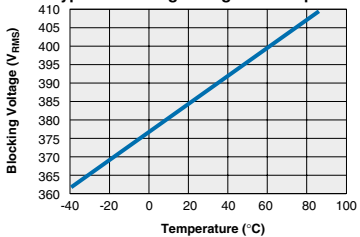
LBA110L - FormB Typical Blocking Voltage vs. Temperature
