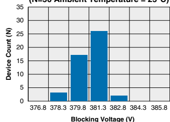
LBA110L - FormA Typical Blocking Voltage Distribution (N=50 Ambient Temperature = 25°C)
