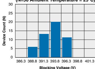
LBA110L - FormB Typical Blocking Voltage Distribution (N=50 Ambient Temperature = 25°C)
