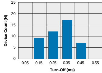
LBA127 - FormA Typical Turn-Off Time (N=50 Ambient Temperature = 25°C) (Load Current = 170mA; I_F = 5\text{mA} )
