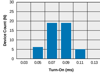
LBA127 - FormB Typical Turn-On Time (N=50 Ambient Temperature = 25°C) (Load Current = 170mA; I_F = 5\text{mA} )
