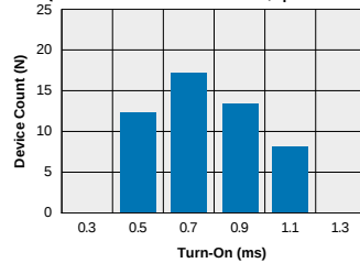
LBA127 - FormA Typical Turn-On Time (N=50 Ambient Temperature = 25°C) (Load Current = 170mA; I_F = 5\text{mA} )
