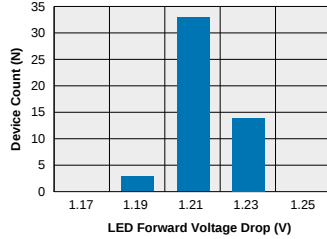
LBA127 Typical LED Forward Voltage Drop (N=50 Ambient Temperature = 25°C; I_F = 5\text{mA} )
