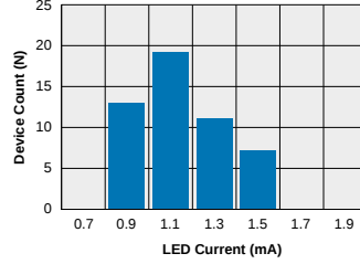
LBA127 - FormA Typical I_F for Switch Dropout (N=50 Ambient Temperature = 25°C) (Load Current = 170mA)
