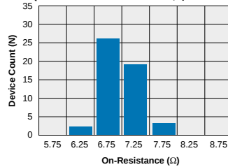
LBA127 - FormA Typical On-Resistance Distribution (N=50 Ambient Temperature = 25°C) (Load Current = 170mA, I_F = 5\text{mA} )
