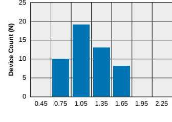
LBA127 - FormB Typical I_F for Switch Dropout (N=50 Ambient Temperature = 25°C) (Load Current = 170mA)
