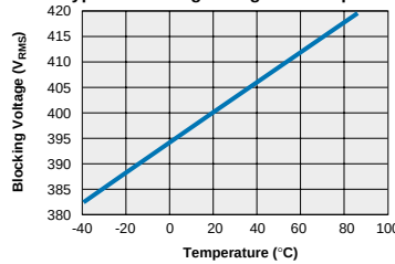
LCC110 - FormB Typical Blocking Voltage vs. Temperature
