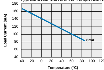
LCC110 - FormB Typical Load Current vs. Temperature
