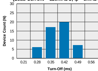
LCC110 - FormB Typical Turn-Off Time (N=50 Ambient Temperature = 25°C) (Load Current = 120mADC; I_F = 8\text{mADC} )
