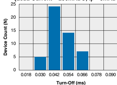
PAA140 Typical Turn-Off Time (N=50 Ambient Temperature = 25°C) (Load Current = 250mADC; I_F = 5\text{mADC} )
