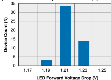
PAA140 Typical LED Forward Voltage Drop (N=50 Ambient Temperature = 25°C; I_F = 5\text{mADC} )
