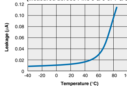
PAA140 Typical Leakage vs. Temperature (Measured across Pins 5 & 6 or 7 & 8)
