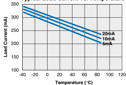
PAA140 Typical Load Current vs. Temperature
