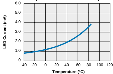
XBA170 - FormB Typical I_F for Switch Operation vs. Temperature (Load Current = 100mADC)
