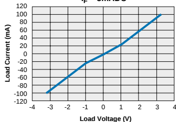
XBA170 - FormB Typical Load Current vs. Load Voltage (Ambient Temperature = 25°C) I_F = 5\text{mADC}
