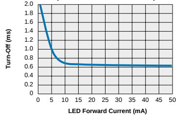
XBA170 - FormB Typical Turn-Off vs. LED Forward Current (Load Current = 100mADC)
