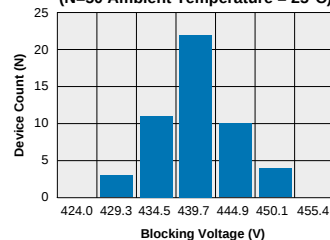
XBA170 - FormB Typical Blocking Voltage Distribution (N=50 Ambient Temperature = 25°C)
