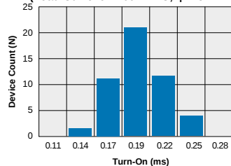
XBA170 - FormB Typical Turn-On Time (N=50 Ambient Temperature = 25°C) (Load Current = 100mADC; I_F = 5mADC)
