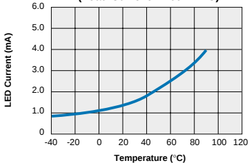
XBA170 - FormA Typical I_F for Switch Dropout vs. Temperature (Load Current = 100mADC)
