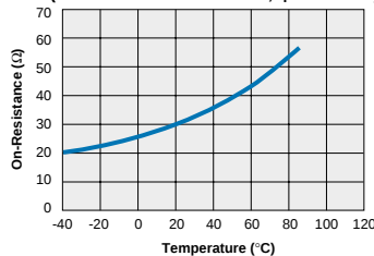
XBA170 - FormA Typical On-Resistance vs. Temperature (Load Current = 100mADC; I_F = 5\text{mADC} )
