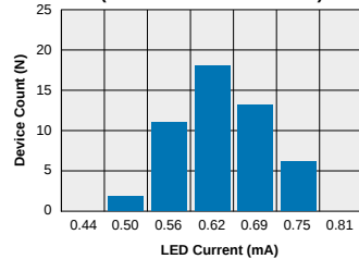
XBA170 - FormA Typical I_F for Switch Dropout (N=50 Ambient Temperature = 25°C) (Load Current = 100mADC)
