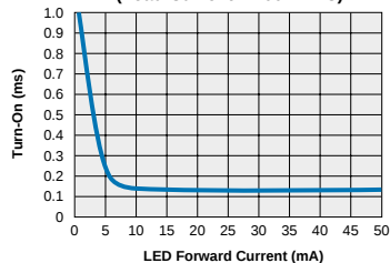
XBA170 - FormB Typical Turn-On vs. LED Forward Current (Load Current = 100mADC)
