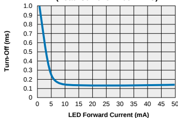
XBA170 - FormA Typical Turn-Off vs. LED Forward Current (Load Current = 100mADC)
