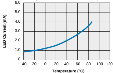
XBA170 - FormA Typical I_F for Switch Operation vs. Temperature (Load Current = 100mADC)
