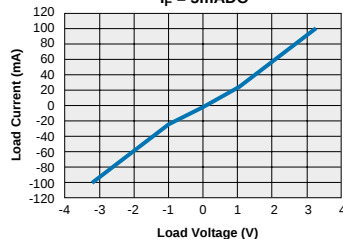
XBA170 - FormA Typical Load Current vs. Load Voltage (Ambient Temperature = 25°C) I_F = 5\text{mADC}
