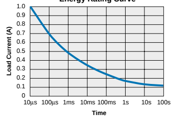
XBA170 Energy Rating Curve
