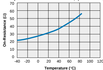
XBA170 - FormB Typical On-Resistance vs. Temperature (Load Current = 100mADC; I_F = 5\text{mADC} )
