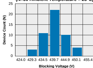
XBA170 - FormA Typical Blocking Voltage Distribution (N=50 Ambient Temperature = 25°C)
