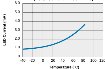
XBA170 - FormB Typical I_F for Switch Dropout vs. Temperature (Load Current = 100mADC)
