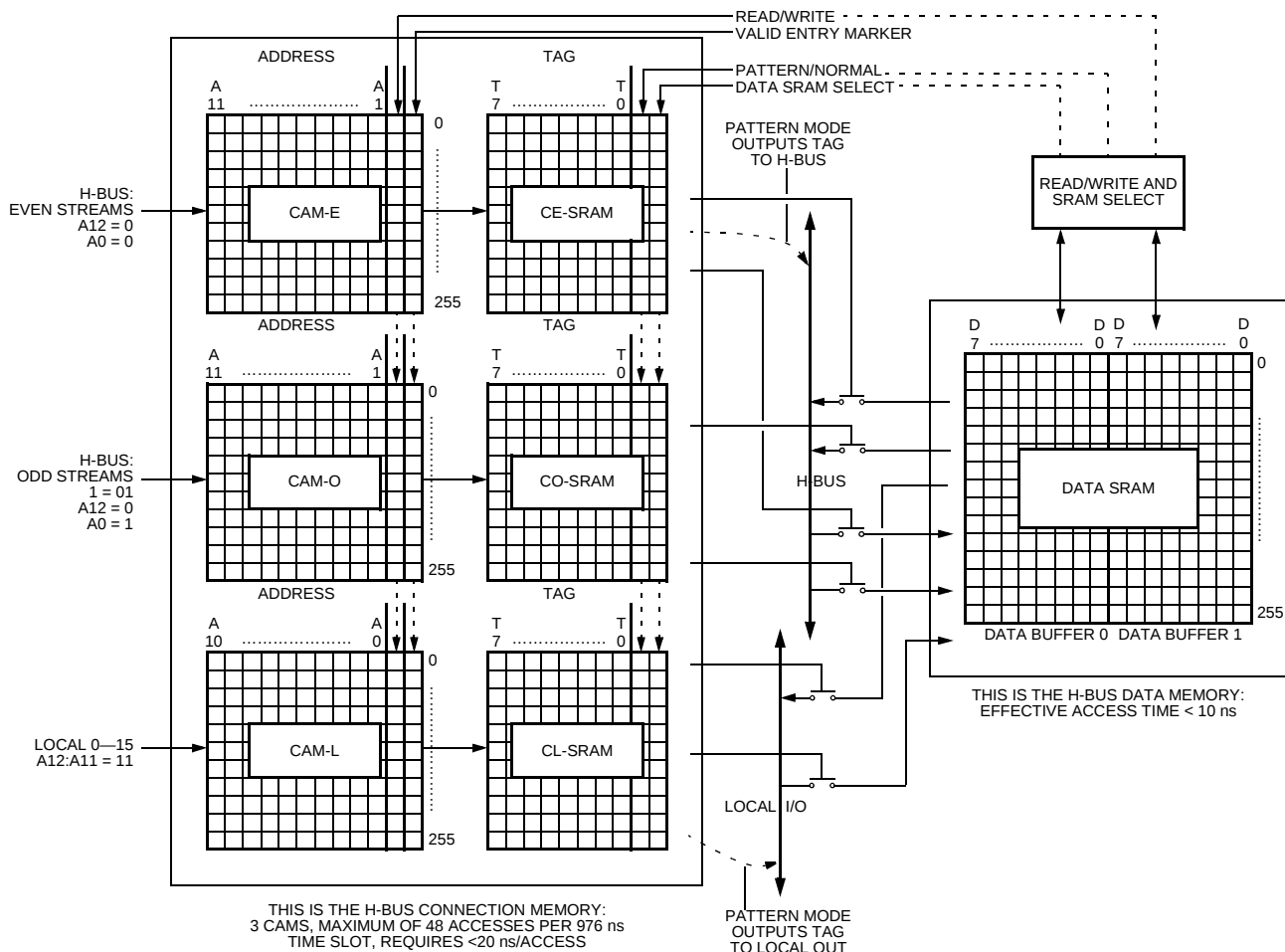
Figure 9. CAM Architecture
