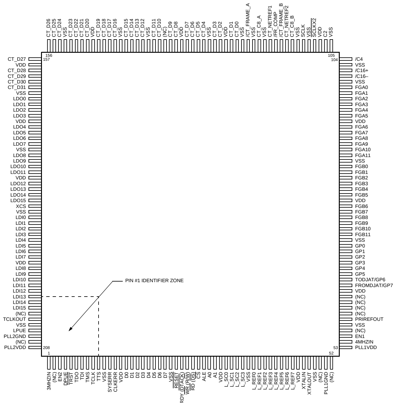
Figure 1. 208 SQFP—Top View
