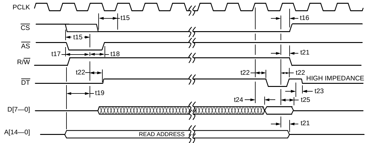
Figure 20. Synchronous Read Cycle Timing
