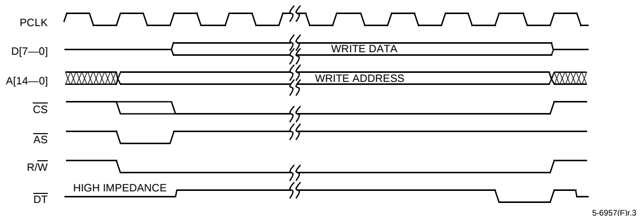
Figure 8. Synchronous Write
