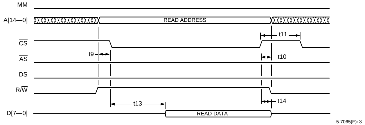
Figure 18. Asynchronous Read Cycle Timing Using Only \overline{CS}
