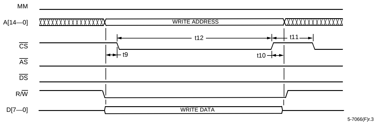
Figure 19. Asynchronous Write Cycle Timing Using Only \overline{CS}
