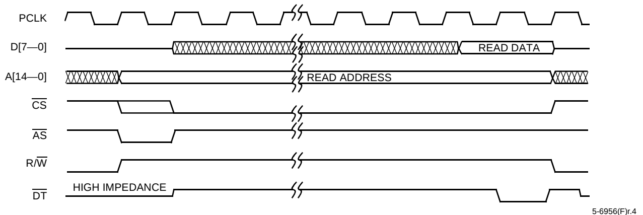
Figure 7. Synchronous Read
