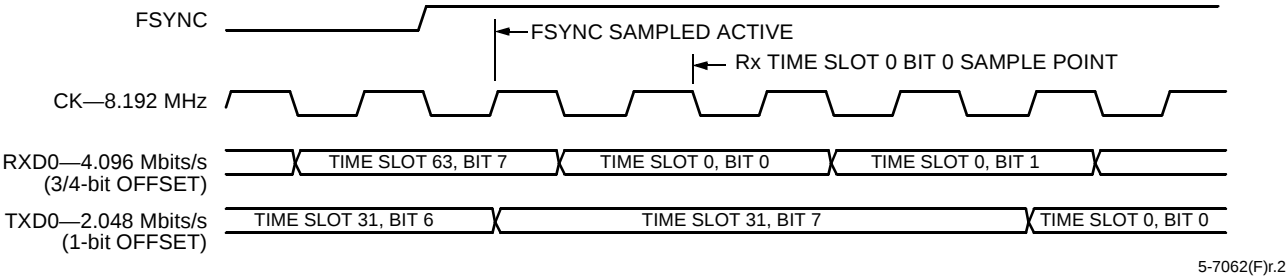
Figure 12. Highway Offsets
