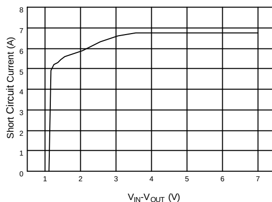
Fig. 6 AIC1084 (ADJ.) Short Circuit Current
