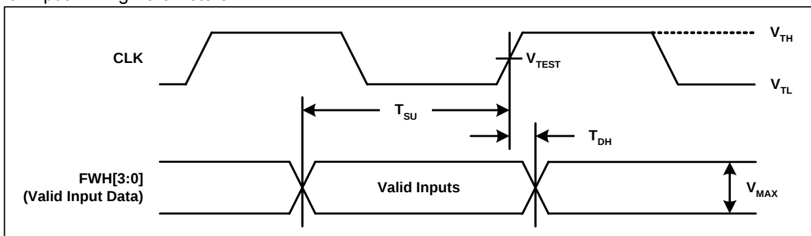
Figure 5: Input Timing Parameters
