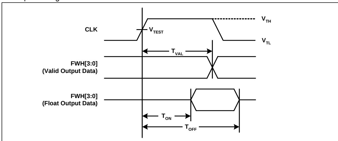
Figure 6: Output Timing Parameters
