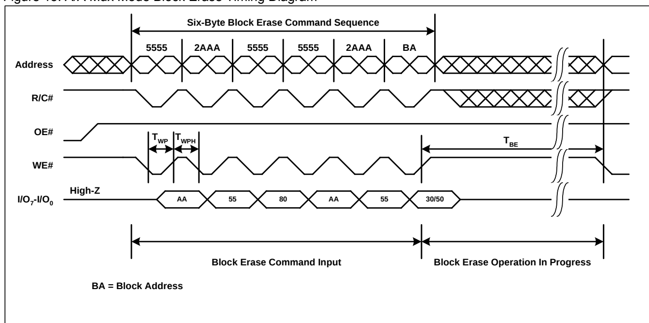
Figure 15: A/A Mux Mode Block Erase Timing Diagram
