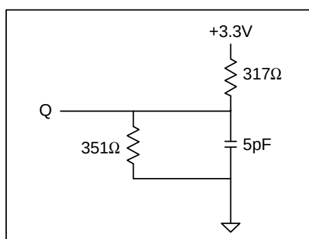
Figure 2 Output Load Equivalent
