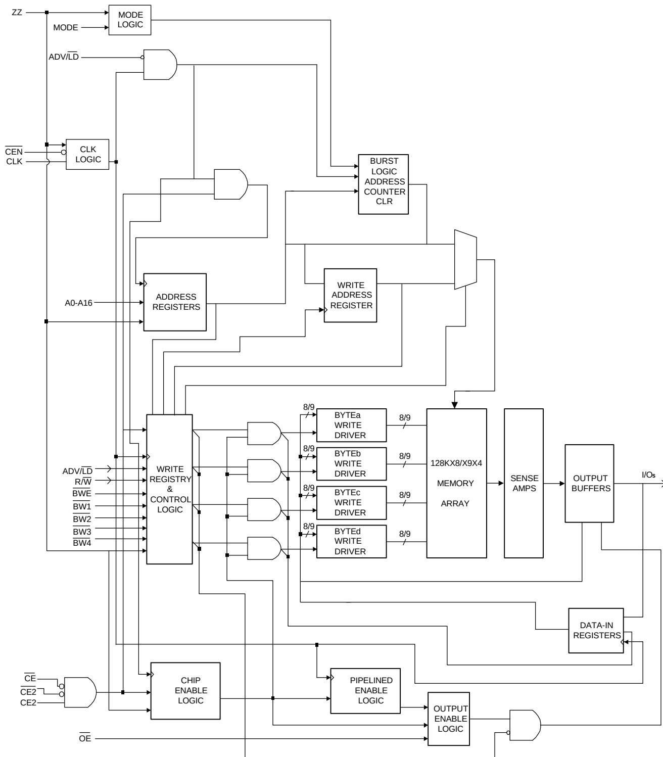
Block Diagram (128K X 32/36)
