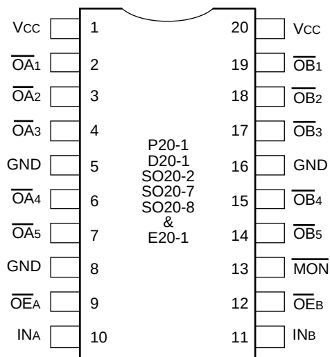
DIP/SSOP/SSOP/SSOP/QSOP/CERPACK TOP VIEW
