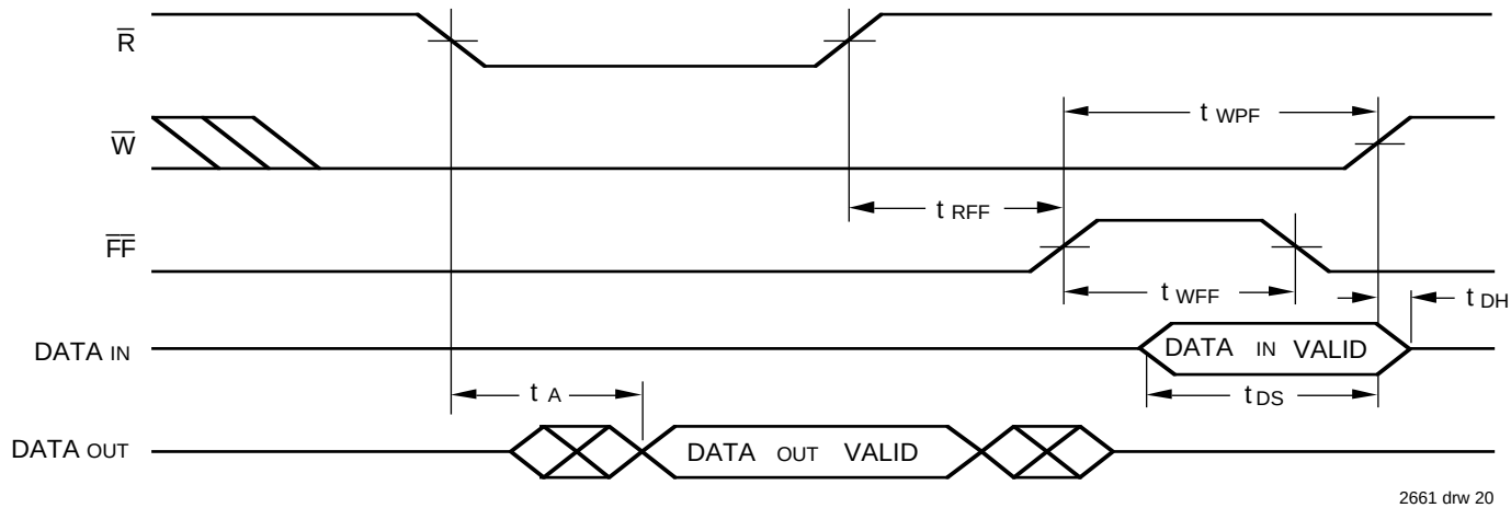
Figure 18. Write Data Flow-Through Mode
