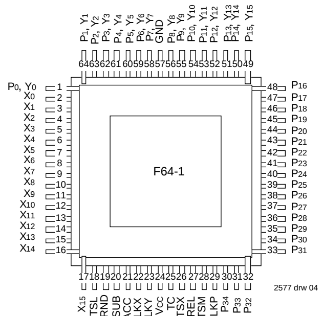
PLCC TOP VIEW
