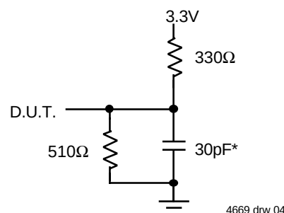
Figure 2. Output Load
