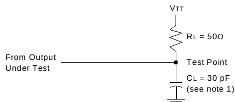
Load Circuit
