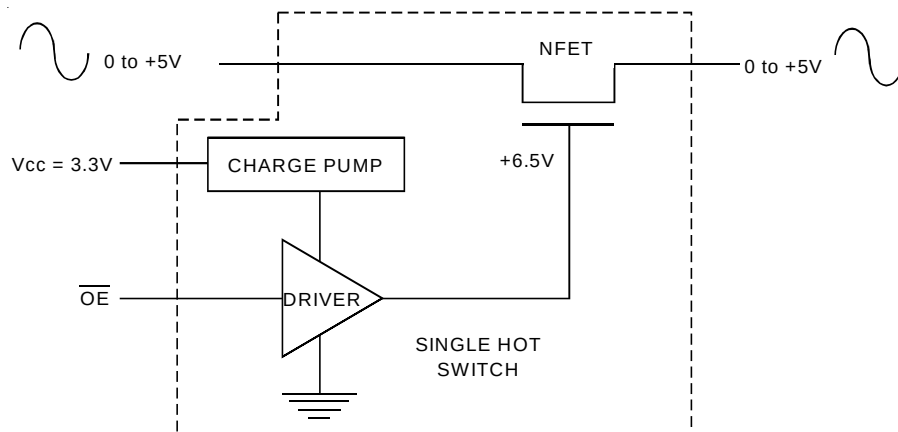
Rail-to-Rail Switching
