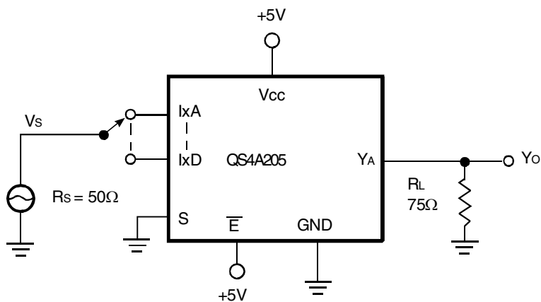
Off-Isolation
