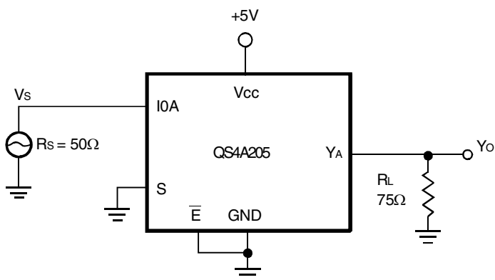
Insertion Loss
