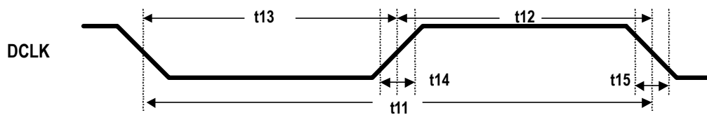
Figure 17. DCLK Timing in Mode '1'
