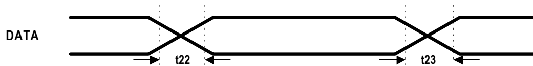
Figure 19. DATA Output Timing in Mode '0'
