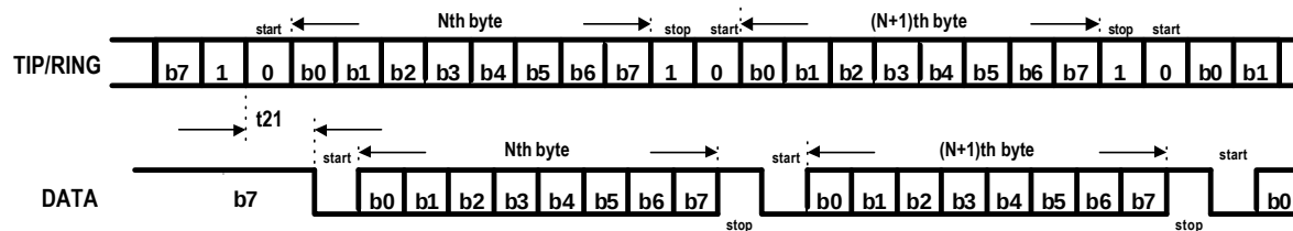
Figure 20. Serial Data Interface Timing in MODE '0'
