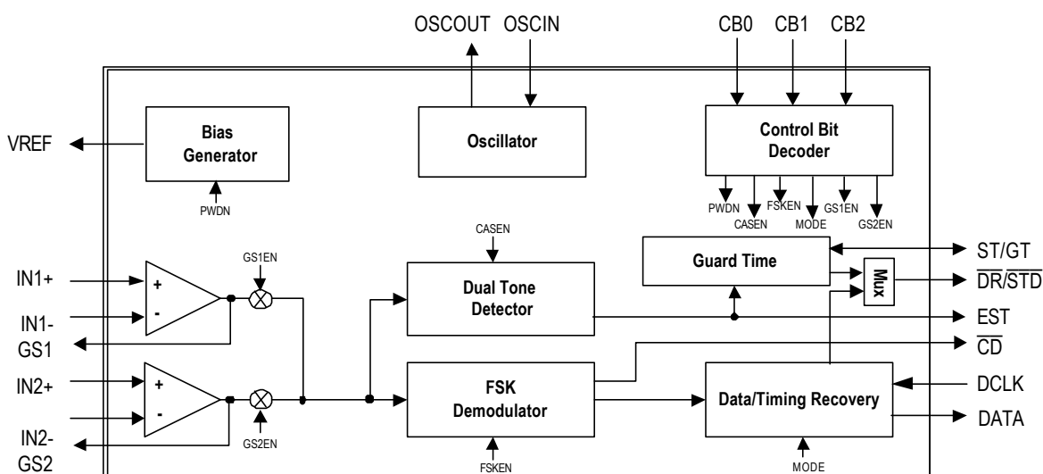
Figure 1. Block Diagram
