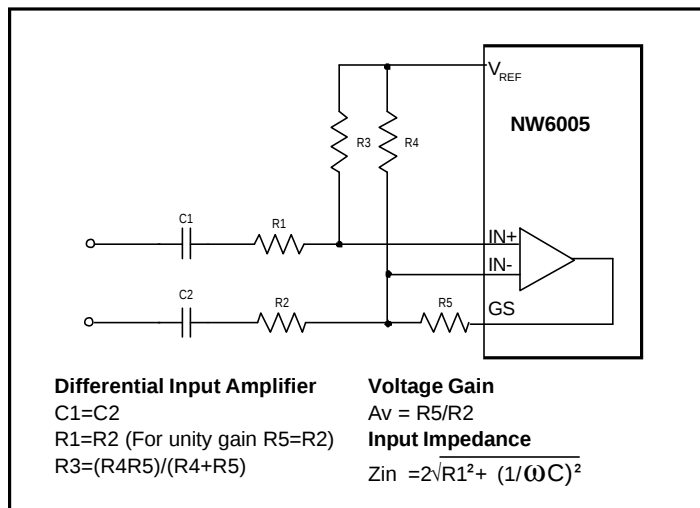
Figure 3. Differential Input Gain Control Circuit
