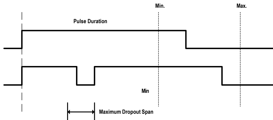
Figure 21. Valid DT-AS Pulses
