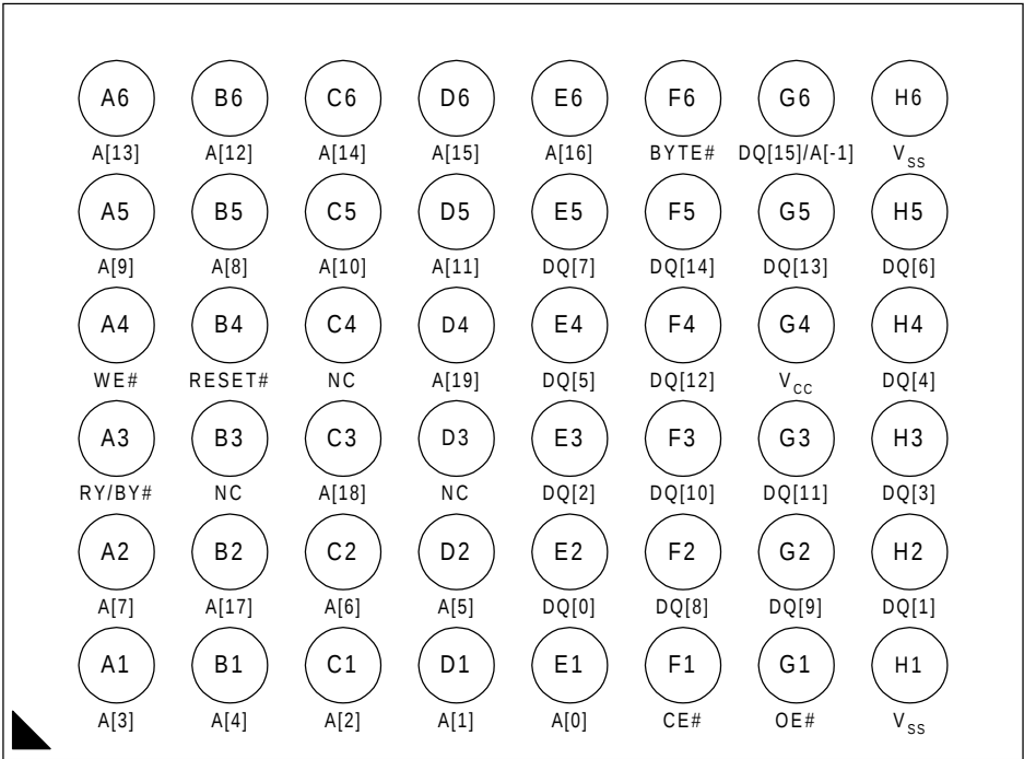
48-Ball FBGA (Top View, Balls Facing Down)
