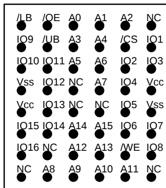
48-FBGA(Top View)
