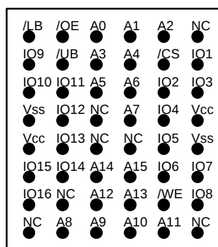
48-FBGA(Top View)
