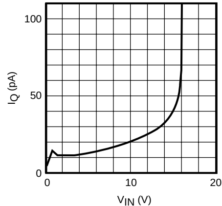
QUIESCENT CURRENT (OFF MODE) vs. INPUT VOLTAGE
