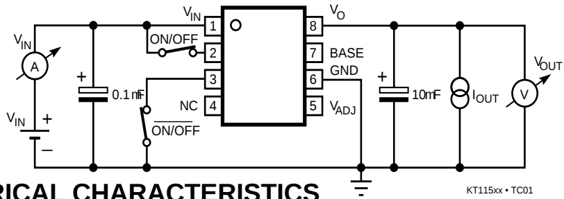
TEST CIRCUIT 1
