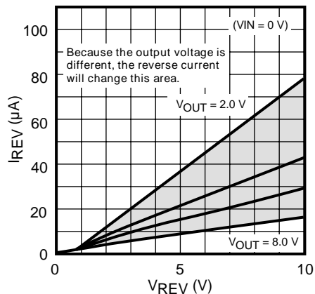
REVERSE BIAS CURRENT RANGE
