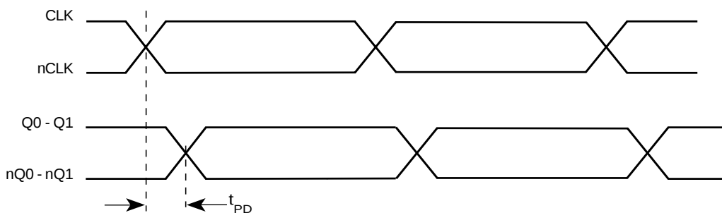
FIGURE 6 - PROPAGATION DELAY
