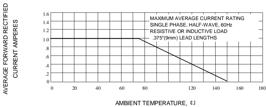
Fig. 5-FORWARD DERATING CURVE
