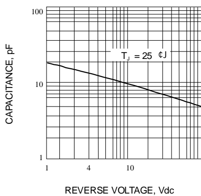
Fig. 4-TYPICAL JUNCTION CAPACITANCE
