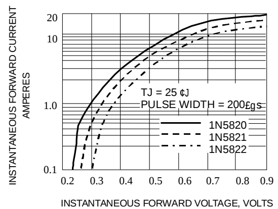
Fig. 4-TYPICAL FORWARD CHARACTERISTICS
