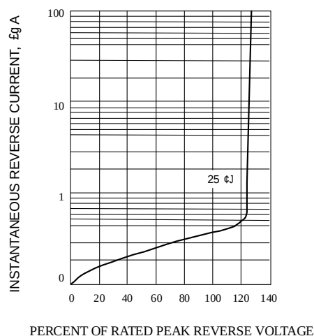
Fig. 4-REVERSE CHARACTERISTICS
