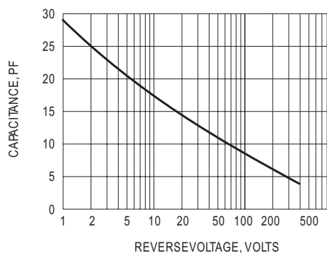
Fig.5-TYPICAL JUNCTION CAPACITANCE
