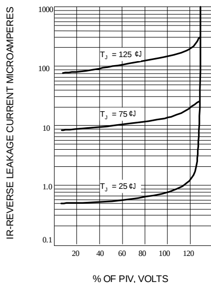
Fig. 5-TYPICAL REVERSE CHARACTERISTICS
