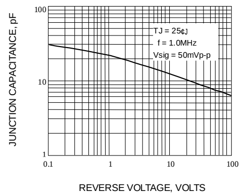
Fig. 6-TYPICAL JUNCTION CAPACITANCE
