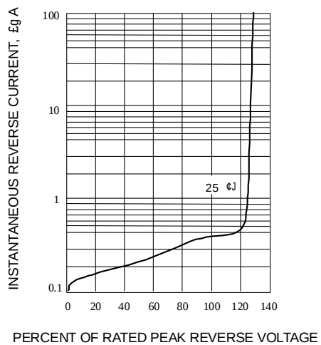
Fig. 1-TYPICAL REVERSE CHARACTERISTICS
