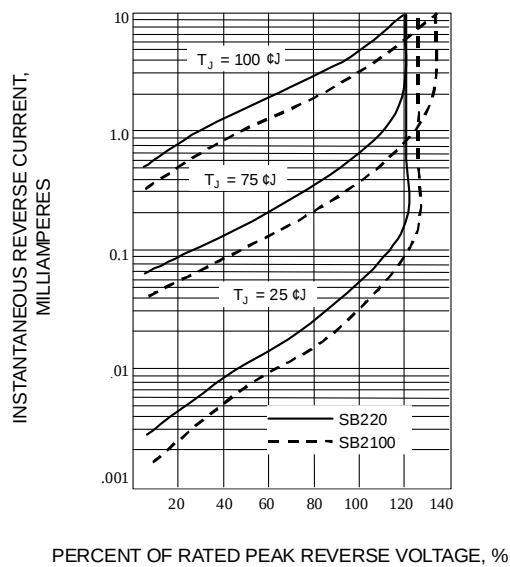
Fig. 3-TYPICAL REVERSE CHARACTERISTICS
