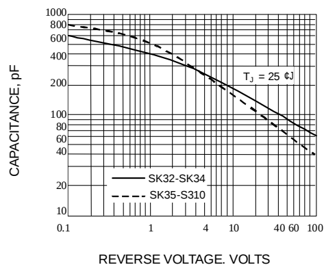
Fig. 4-TYPICAL JUNCTION CAPACITANCE
