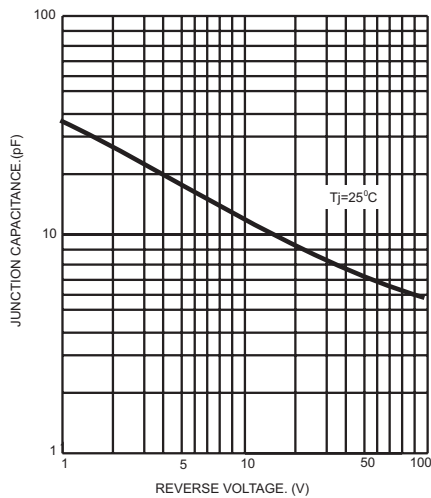
FIG.2- TYPICAL JUNCTION CAPACITANCE
