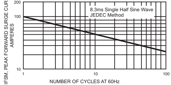
FIG.4- MAXIMUM NON-REPETITIVE FORWARD SURGE CURRENT UNIDIRECTIONAL ONLY
