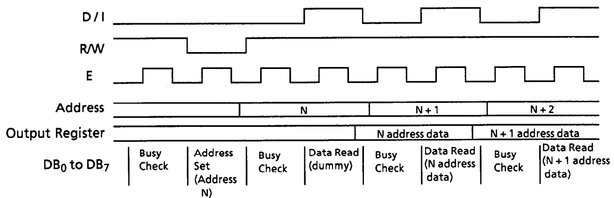
Figure 4 Read Timing
