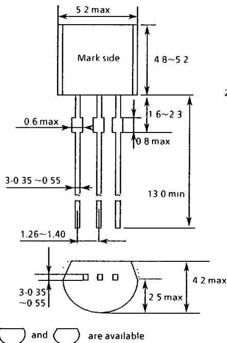
Figure 7 Dimensions
