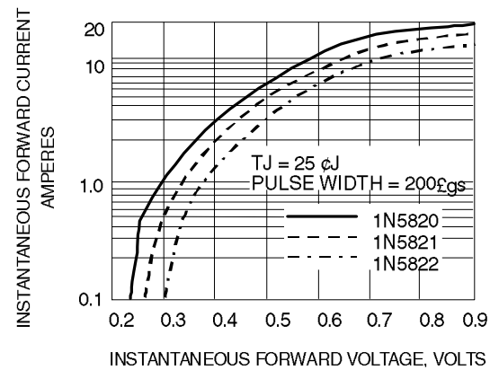
Fig. 4-TYPICAL FORWARD CHARACTERISTICS
