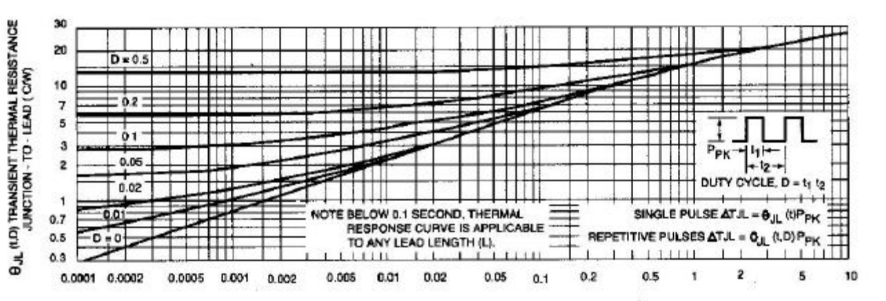
Fig. 2-TYPICAL THERMAL RESPONSE L
