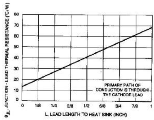
Fig. 10-TYPICAL THERMAL RESISTANCE
