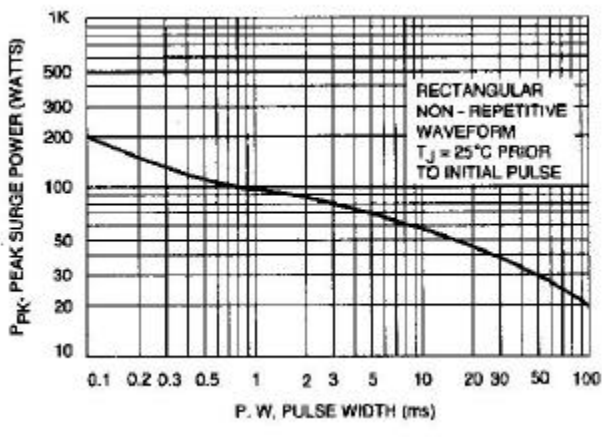
Fig. 3-MAXIMUM SURGE POWER
