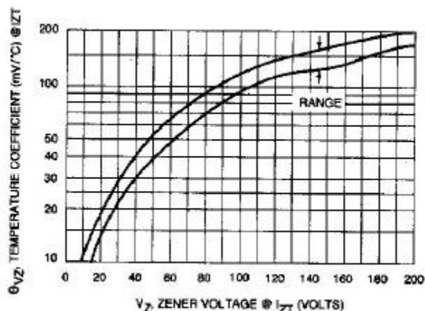
Fig. 6-UNITS 10 TO 200 VOLTS
