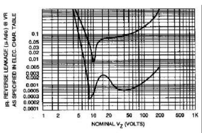
Fig. 4-TYPICAL REVERSE LEAKAGE
