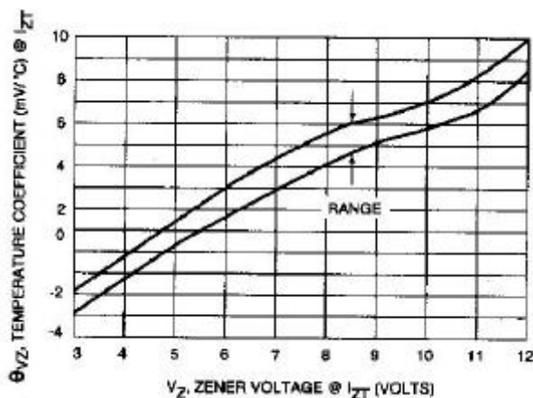
Fig. 5-UNITS TO 12 VOLTS
