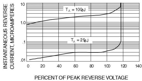
Fig. 3-TYPICAL REVERSE CHARACTERISTICS
