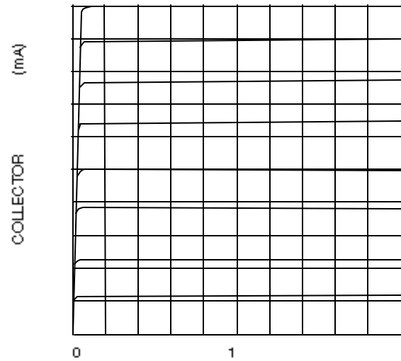
COLLECTOR-EMITTER Emitter-Collector Characteristics
